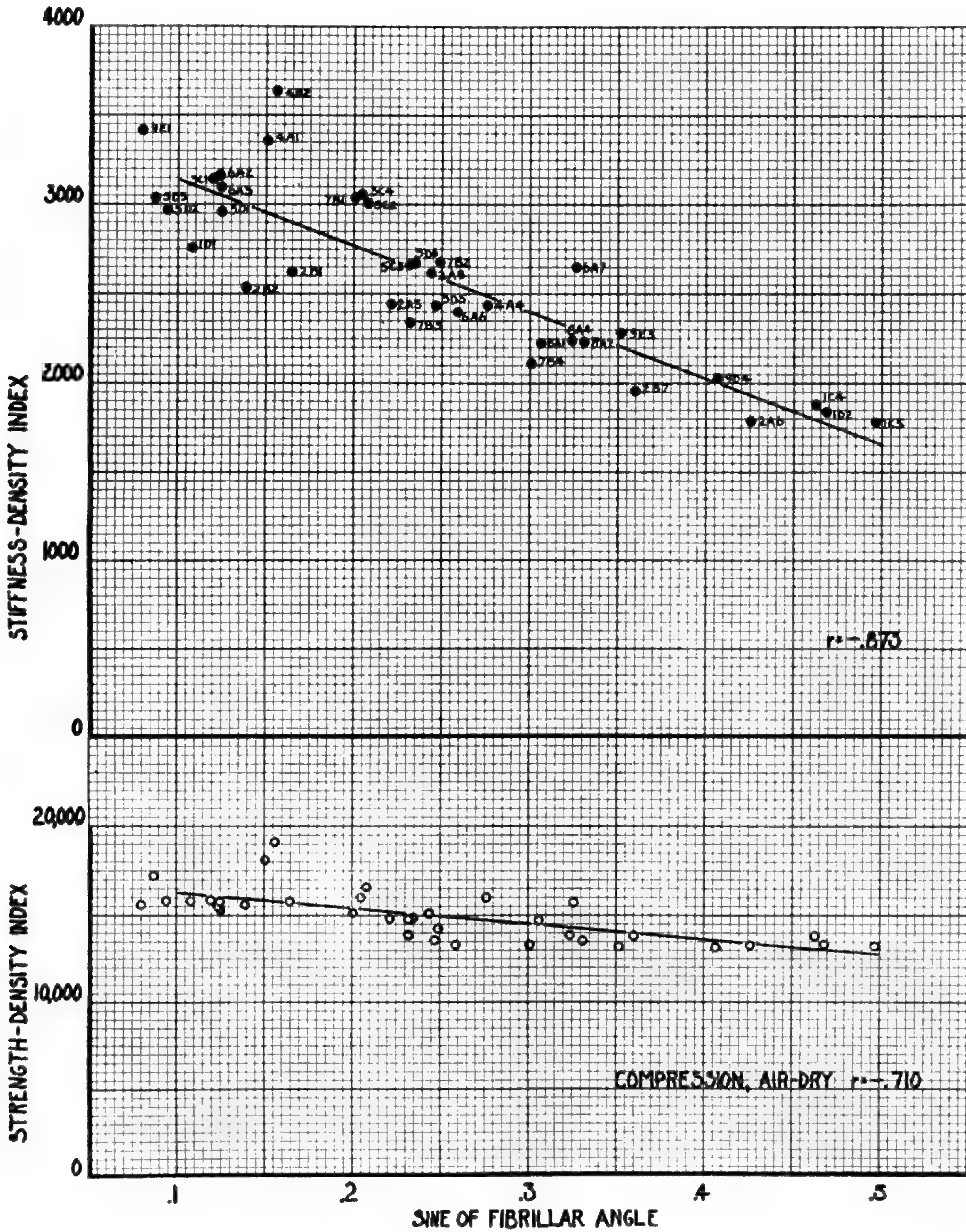
Fig. 15. Axial compression strength-density index (ultimate strength ÷ specific gravity) and stiffness-density index (modulus of elasticity ÷ specific gravity) correlated with sine of average fibrillar angle in summerwood for air-dry specimens.
